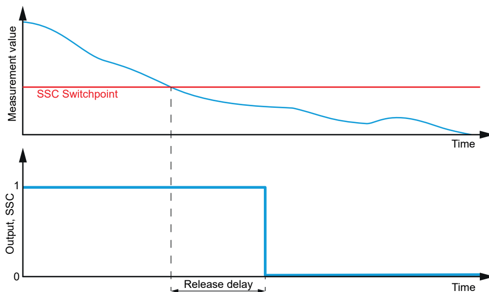
Abb. 13: Release Delay
