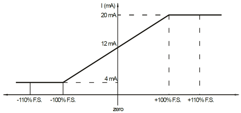
插图 7: Out.mA = 4 - 20 - 0 +
