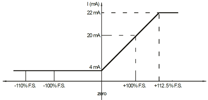
插图 6: Out.mA = 4 - 22 +
